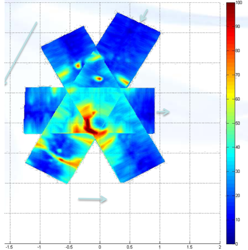
HIRAD 5 GHz excess T_b filtered 16 Sep Karl legs 2, 4 and 6, 65 deg
