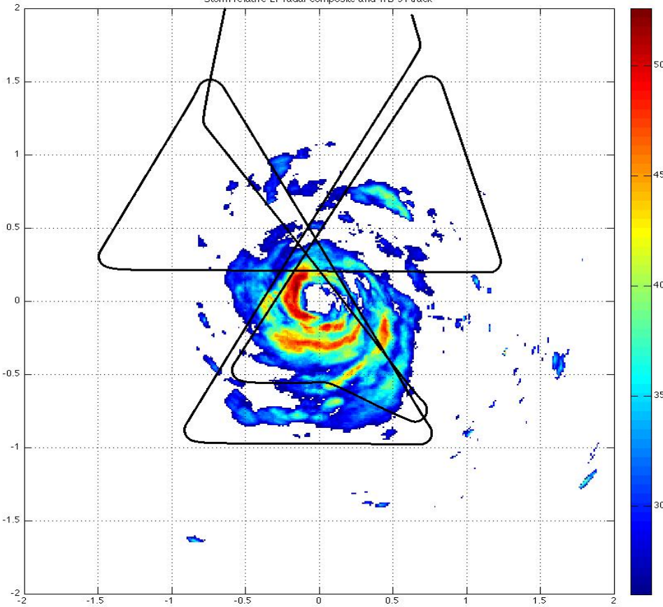
Storm-relative LF radar composite and WB-57 track
